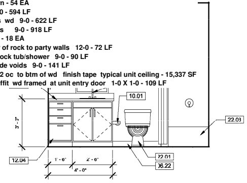
4 UNIT C-1 BATHRM ELEV 3/8" = 1'-0"
