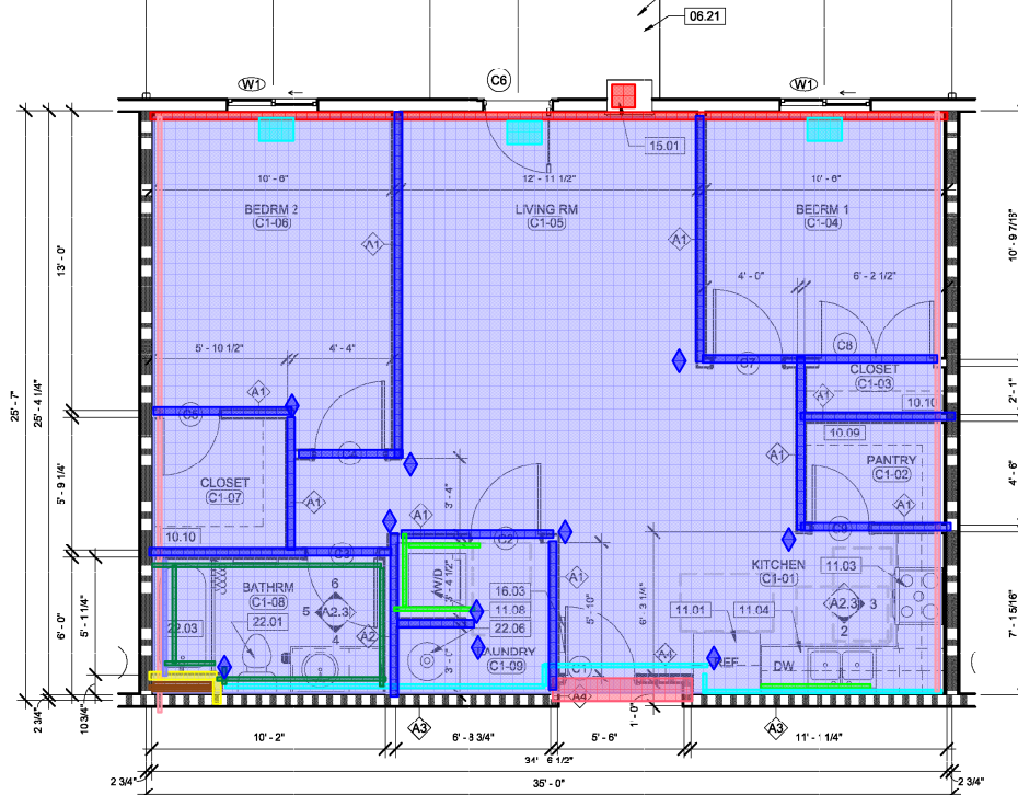
1 UNIT PLAN C-1 1/4" = 1'-0"
