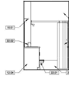
5 UNIT C-1 BATHRM ELEV 3/8" = 1'-0"
