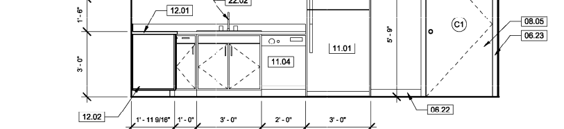
1 KITCHEN ELEV
